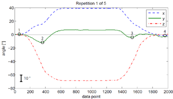
Figure 3. Single trajectory of the dominant arm, with the four characteristic points indicated by black circles.
